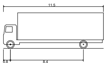
Design Vehicle - TAC HSU (Heavy Single Unit)
