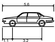
Design Vehicle - TAC P CAR
